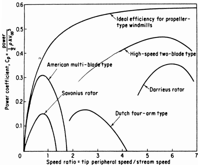
Fig. 5. Typical performance of wind power machines.
