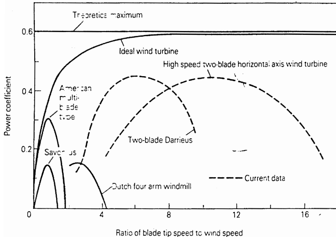
Figure 13.2 Wind turbine power coefficients
