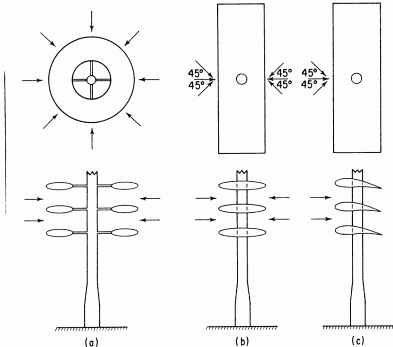
Fig. 35. Three versions of the wing aerogenerator: (a) The circular neutral wing aerogenerator. (b) The linear neutral wing aerogenerator. (c) The linear lift wing aerogenerator. The aspirator holes in the wings are not shown.
