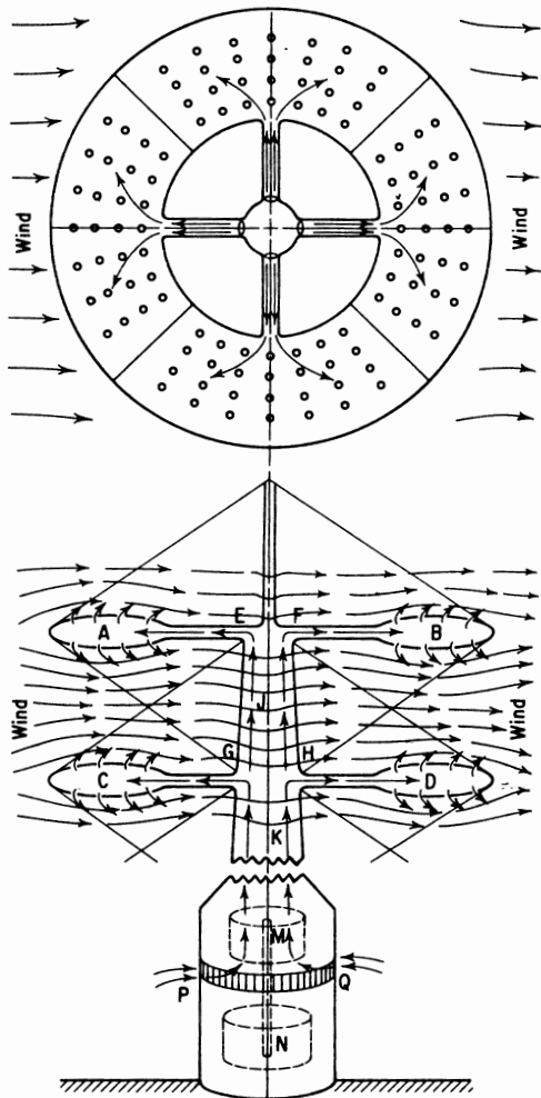
Fig. 34. The circular neutral wing aerogenerator. This aerogenerator has been described in a document submitted by E. Wendell Hewson and received on February 4, 1974, by the U.S. Patent Office, which assigned Disclosure Document No. 028124 to it.
