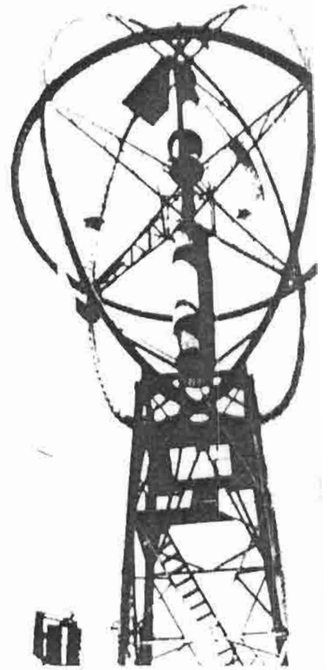
Fig 1d An original 20 kw wind turbine storied one bladed Darrieus rotor with revolution directions under testing at B Moldova
